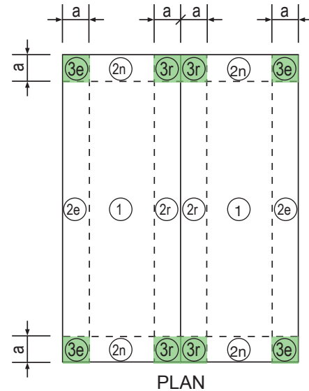
Figure 2.0 Gable Roof Zone Designations
