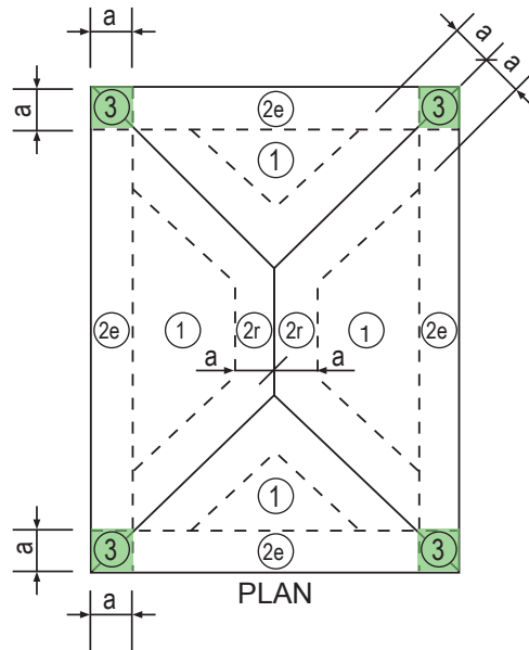
Figure 1.0 Hip Roof Zone Designations
